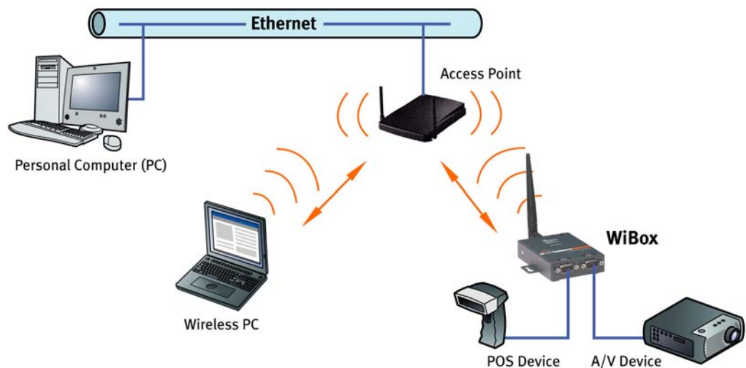
Figure 2-1. Serial Tunneling Infrastructure Network Example
