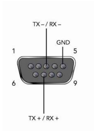
Figure 2-7. RS-485 2-Wire Pinouts
