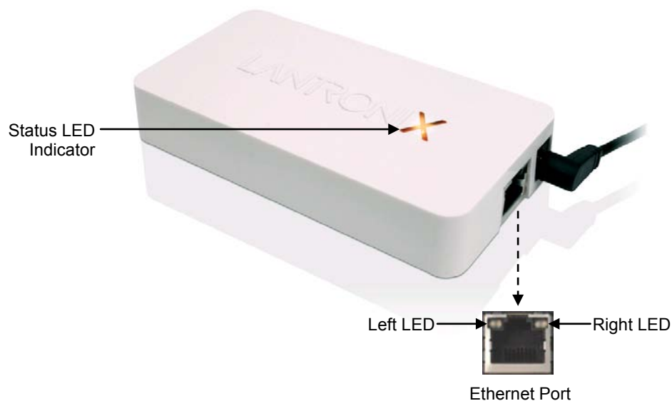
Figure 2-1 xPrintServer LEDs
