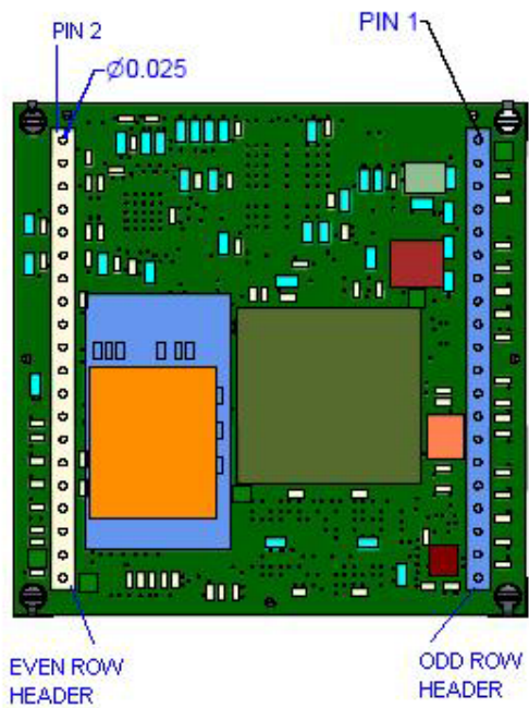
Figure 2-14. Bottom View
